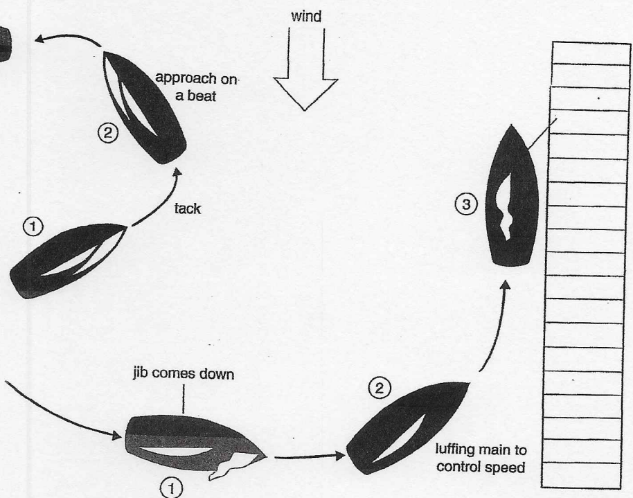
Docking when the wind is blowing parallel with the dock.
