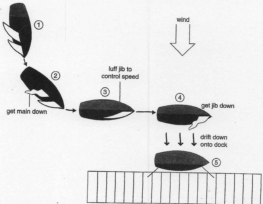
Docking when the dock is downwind.
